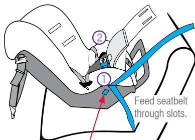
Blue REARWARD FACING BELT PATH label
